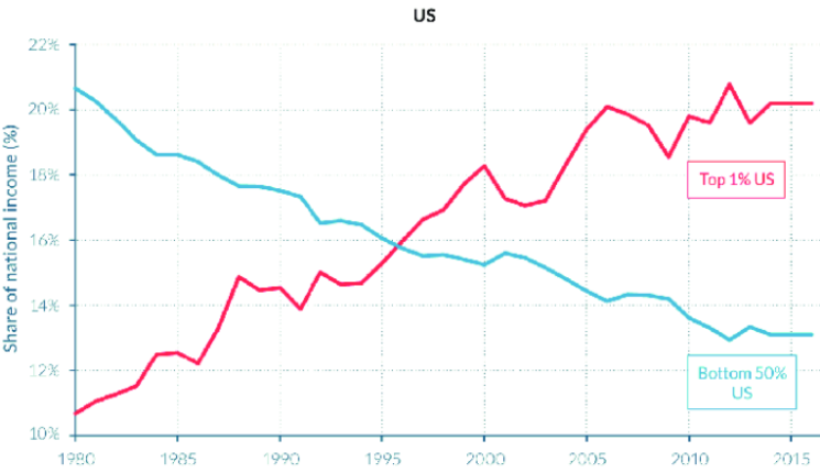
Income inequality in the USA (1980-2016) (WID.world, 2017, see http://wir2018.wid.world/methodology.html for data series and notes )
